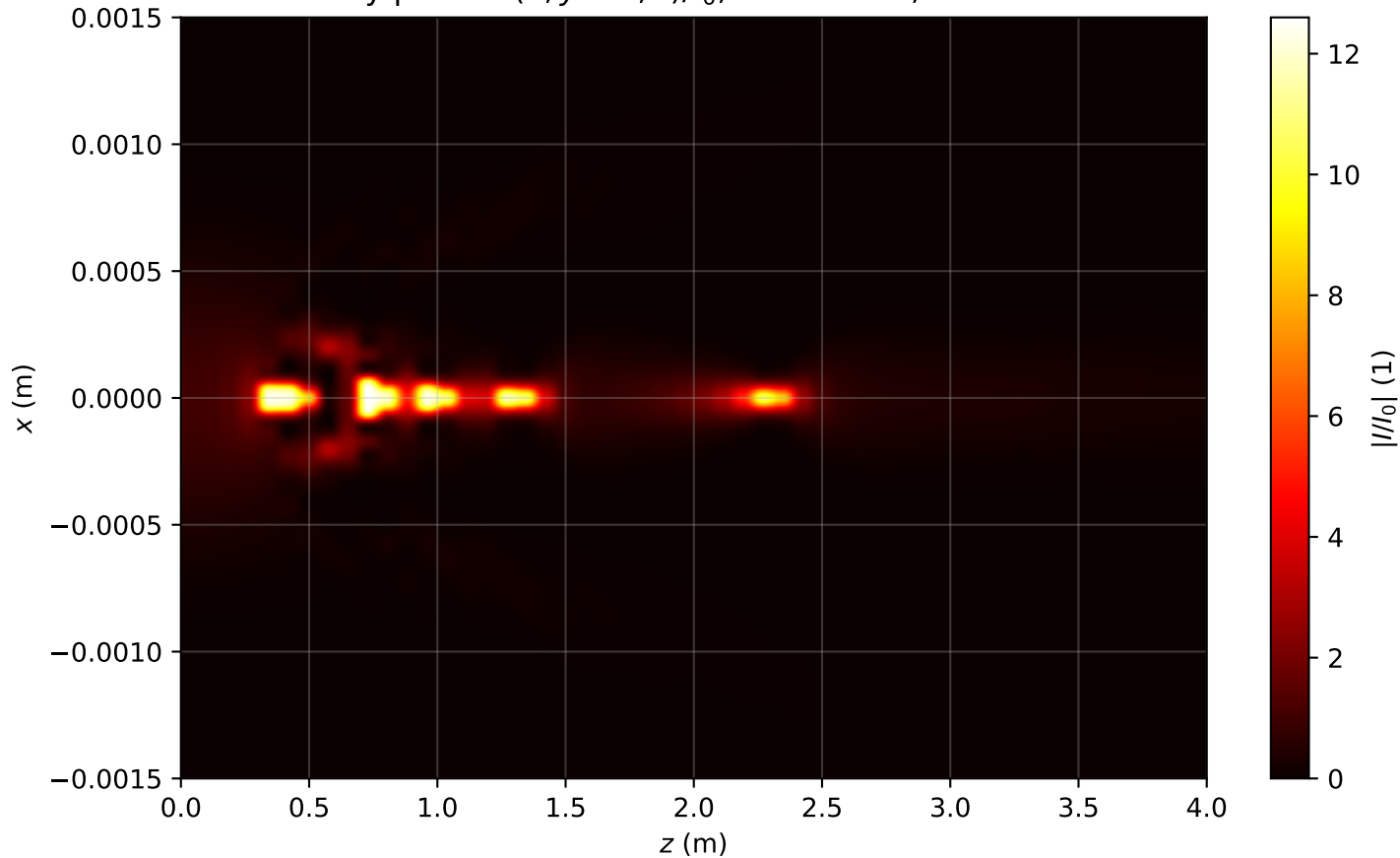
Intensity profile I(x, y = 0, z)/I_0 , P_{in}=9.0P_{cr} , artificial time
